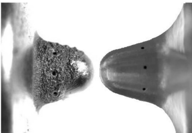
Diesel injector before and after clean up
