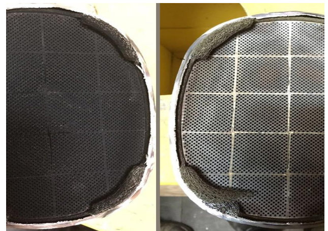
Diesel Particulate Filter before and after clean up
